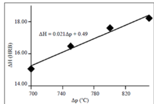
Figure 9: Hardness as a linear function of pouring temperature.
