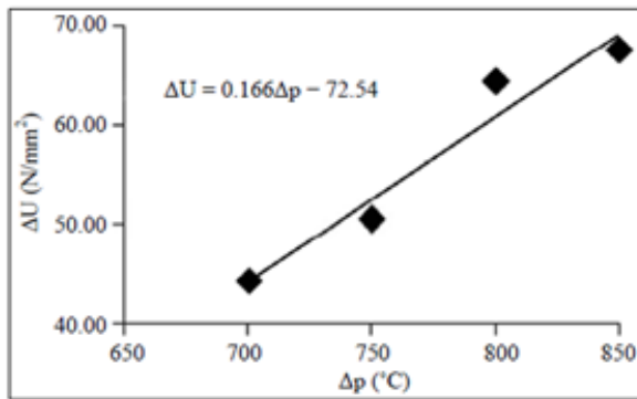
Figure 6: UTS as a linear function of pouring temperature.
