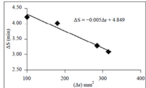
Figure 1: Solidification time as a linear function of runner size.
