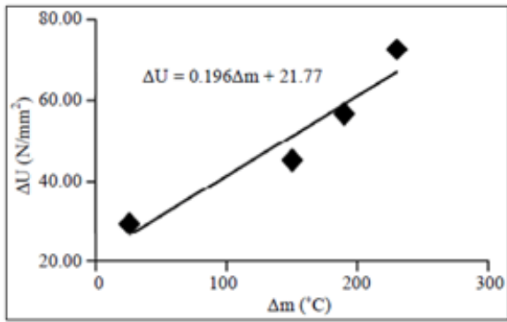
Figure 5: UTS as a linear function of mould temperature.
